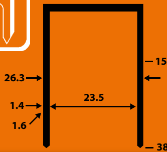
GRAPA SSD □ 1.4 x 1.6 mm
