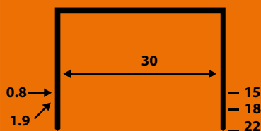
GRAPA CARTÓN C32 □ 0.8 x 1.9 mm
